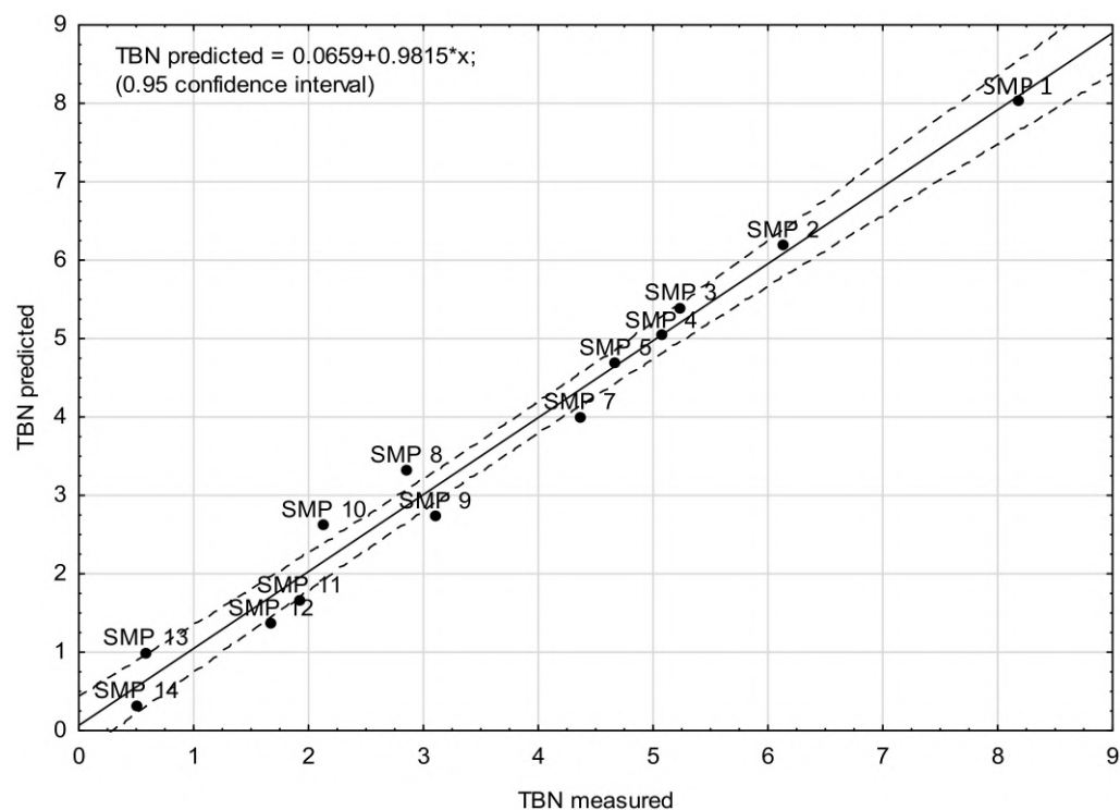
Figure A1. Measured vs. predicted value of TBN (Model A).
