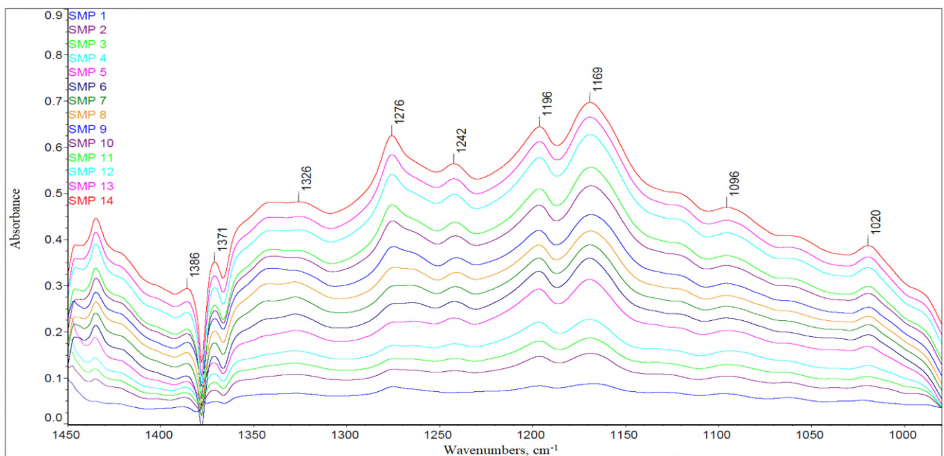
Figure 4. The FTIR differential spectra for the samples, the regions 1000 – 1450\text{ cm}^{-1} .
