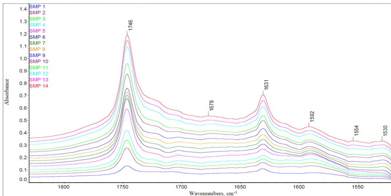
Figure 2. The FTIR differential spectra for the samples of the regions 1475–1800 \text{cm}^{-1} .
