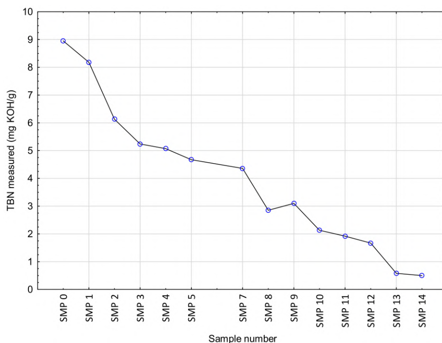
Figure 5. Changes in the TBN of engine oils.
