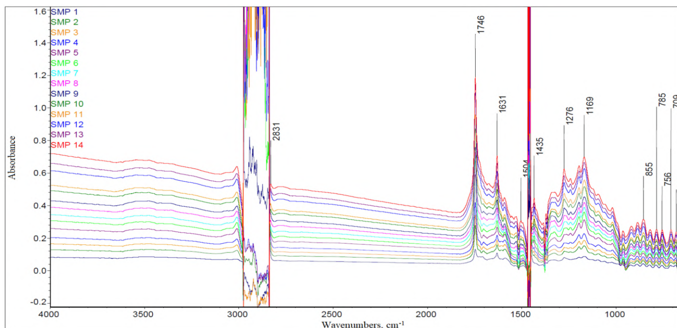
Figure 1. The FTIR differential spectra for the samples of the regions 650–4000 \text{cm}^{-1} .
